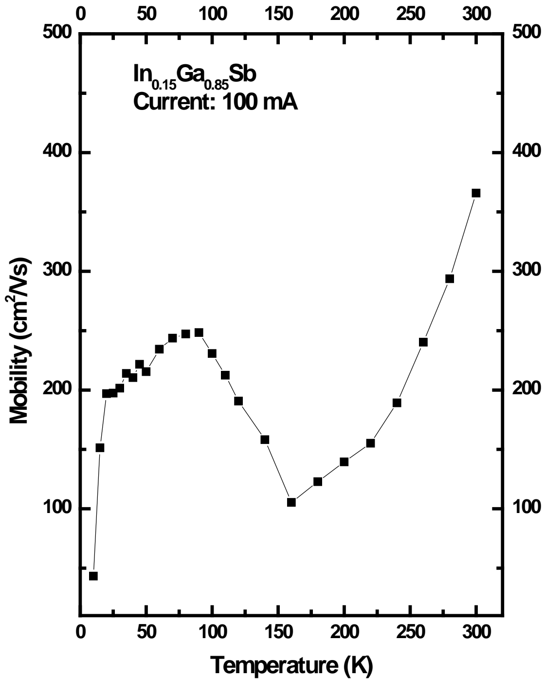
Figure 16. Hall mobility as a function of temperature from In 0.15 Ga 0.85 Sb using a current of 100 mA.
