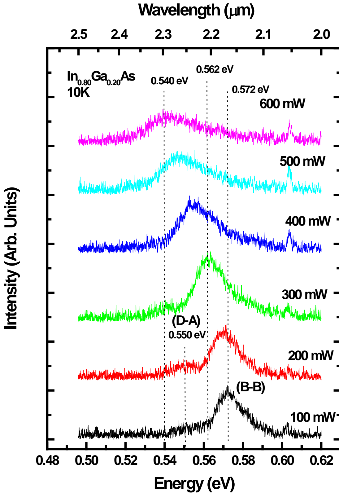
Figure 31. PL data for \text{In}_{0.80}\text{Ga}_{0.20}\text{As} taken at 10 K on location A.
